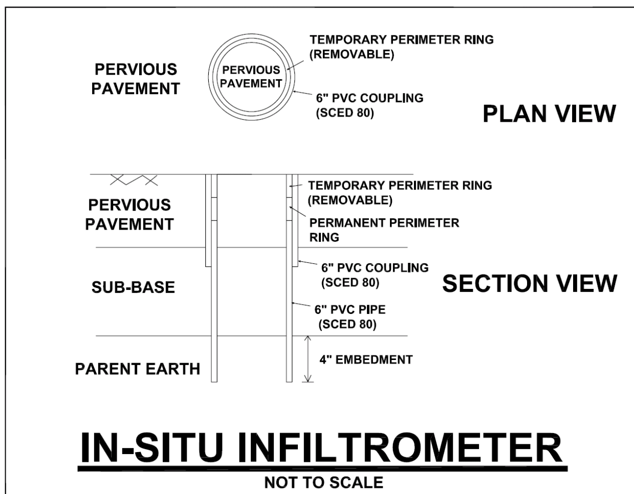
Figure 11.5 Plan View of ERIK In-Situ Infiltrrometer (Embedded Ring Infiltration Kit)
