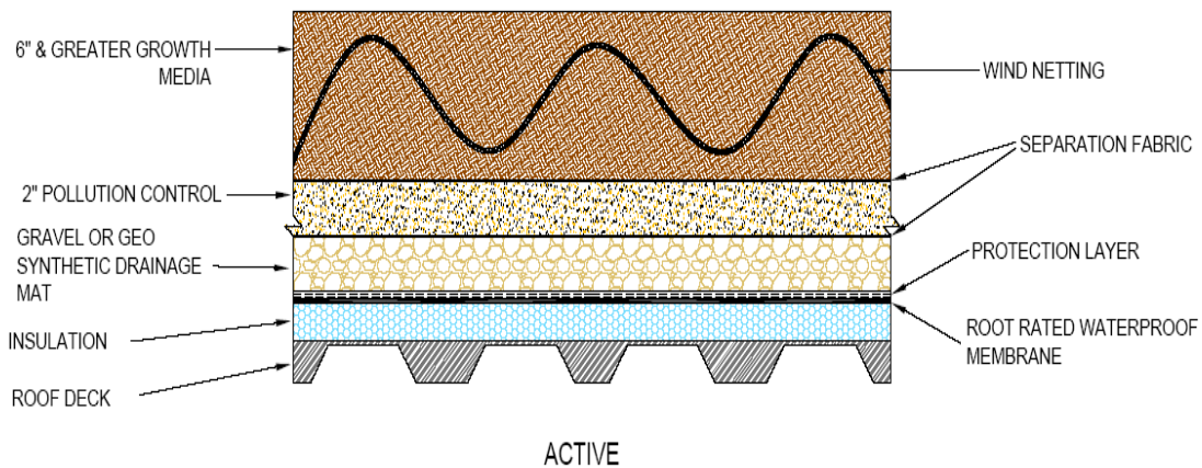
Figure 12.1b Intensive Greenroof Section (Usually Active Function)
