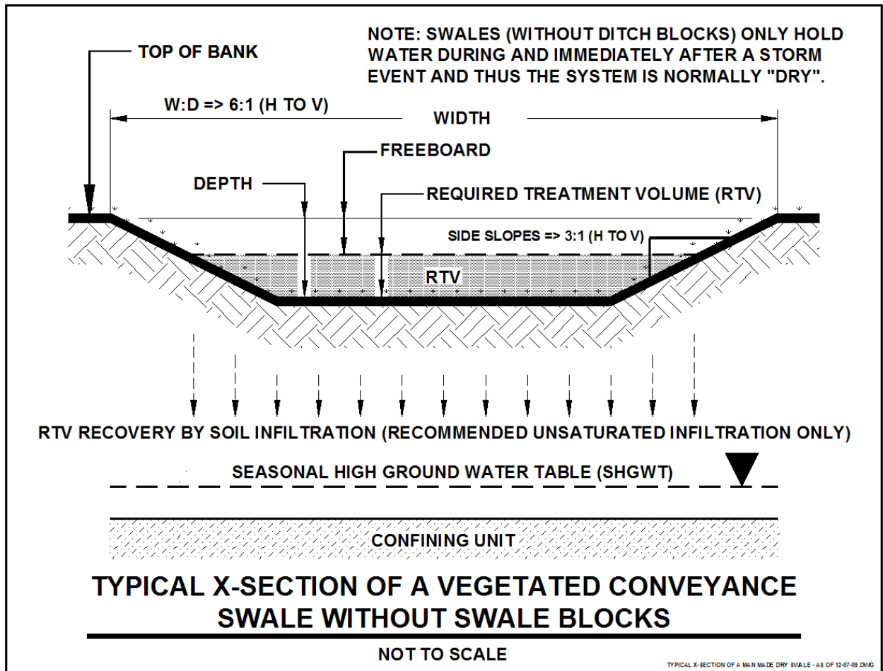
Figure 9.1 Typical Cross-section of a Conveyance Swale without Swale Blocks
