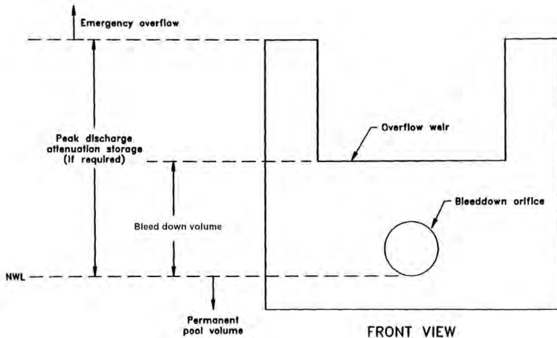
Figure 13.4a Typical Wet Detention Outfall Structure (N.T.S.)
