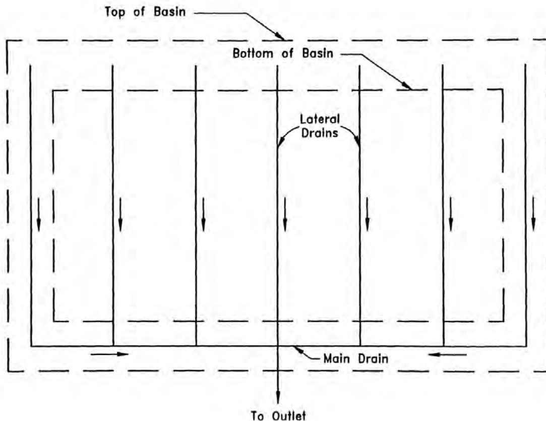
Figure 17.2 Top View of Underdrain System (N.T.S.)
